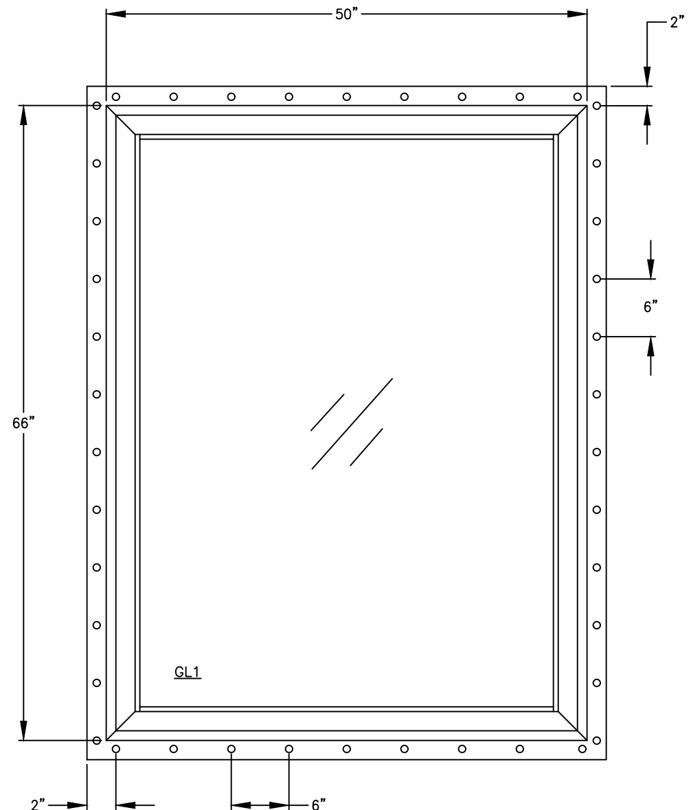
ASPECT/ENDURE FIXED WINDOW (NON-IMPACT) MAXIMUM SIZE: 50" X 66" DESIGN PRESSURE: +50/-50 PSF NAIL FIN INSTALLATION METHOD
