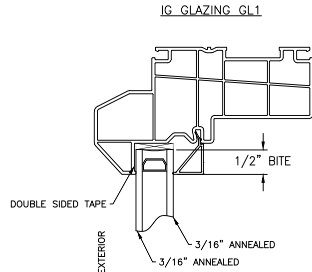
ASPECT/ENDURE FIXED WINDOW (NON-IMPACT) MAXIMUM SIZE: 65" X 79" DESIGN PRESSURE: +50/-50 PSF THRU-FRAME INSTALLATION METHOD
