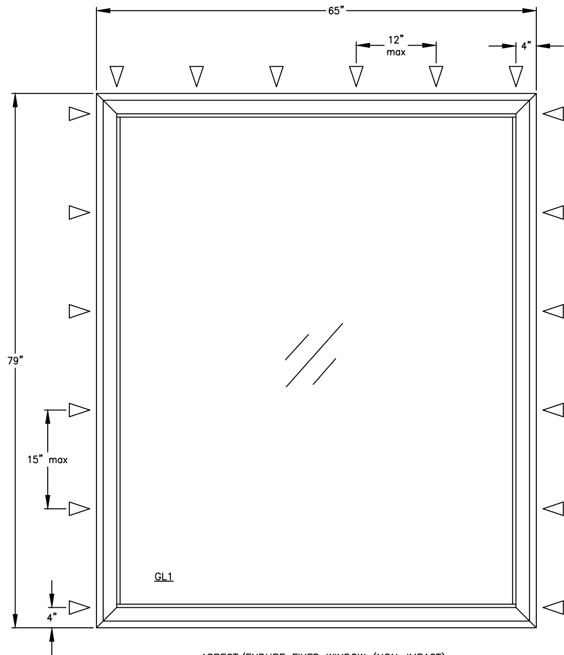
ASPECT/ENDURE FIXED WINDOW (NON-IMPACT) MAXIMUM SIZE: 65" X 79" DESIGN PRESSURE: +50/-50 PSF THRU-FRAME INSTALLATION METHOD
