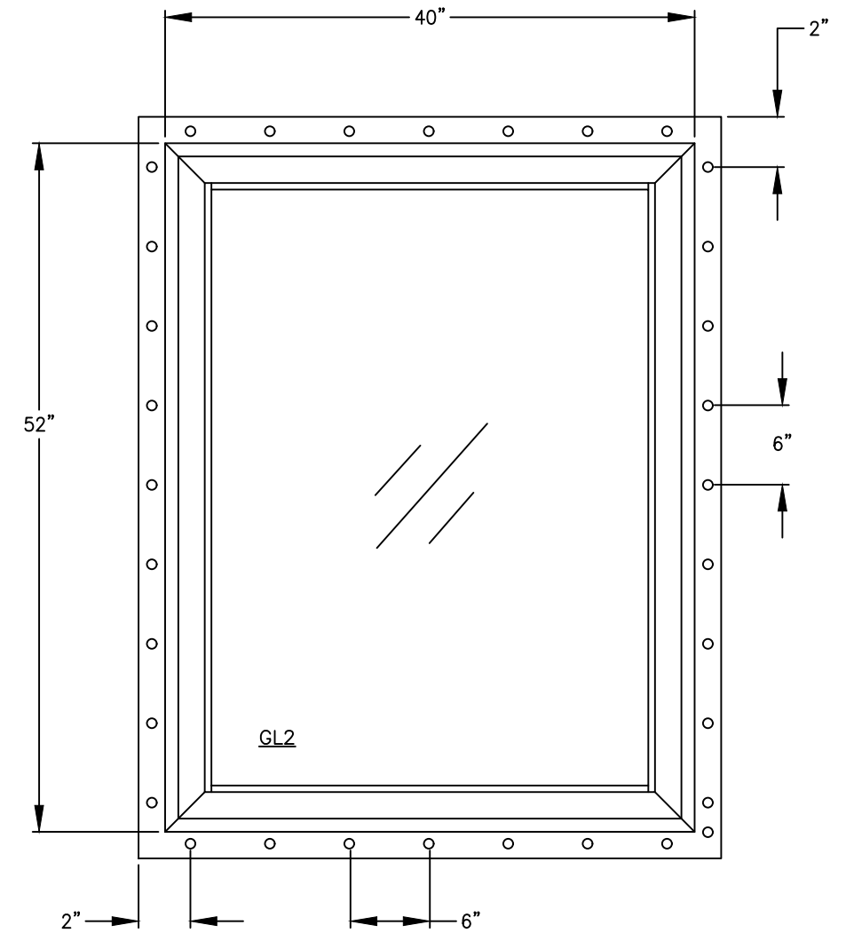
ASPECT/ENDURE FIXED WINDOW (NON-IMPACT) MAXIMUM SIZE: 40" X 52" DESIGN PRESSURE: +55/-55 PSF NAIL FIN INSTALLATION METHOD
